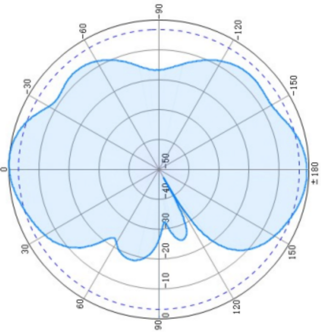
Vertical plane
